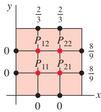
FIGURE 16.1.3 Square region R for Example 1
