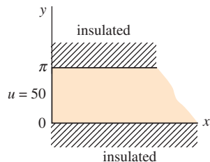
FIGURE 13.R.3 Semi-infinite plate in Problem 8
