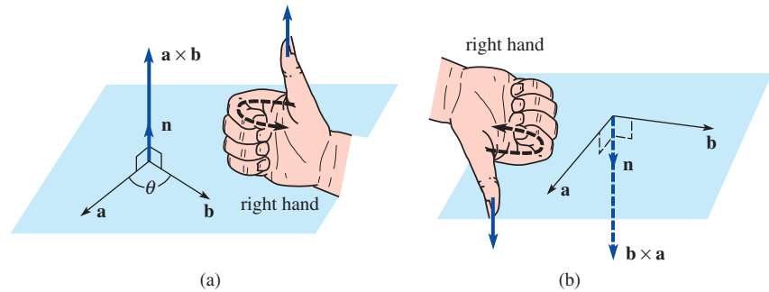
FIGURE 7.4.2 Right-hand rule
