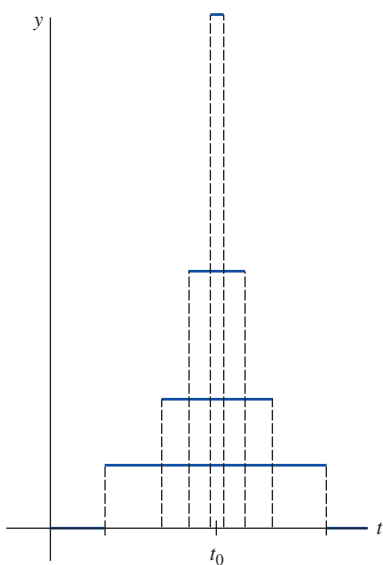
(b) Behavior of \delta_a as a \rightarrow 0
