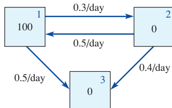
FIGURE 8.17.7 Compartments for Problem 3
