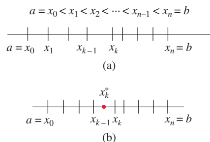
FIGURE 9.8.2 Sample point in k th subinterval
