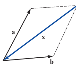
FIGURE 7.1.14 Vector \mathbf{x} in Problem 37
