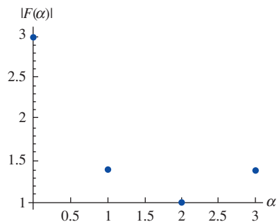
FIGURE 15.5.2 Graph of |F(\alpha)| in Example 1
