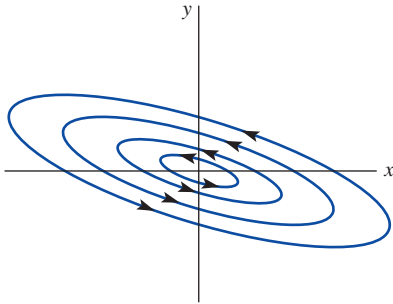
FIGURE 11.2.9 Center
