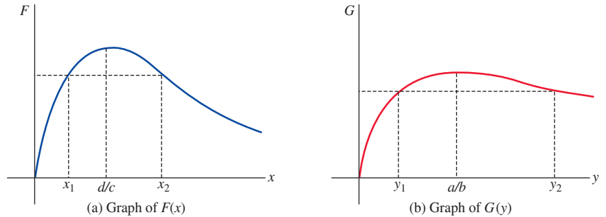
FIGURE 11.4.8 Graphs of F and G help to establish properties 1–3
