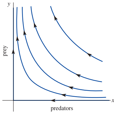
FIGURE 11.4.7 Solutions near (0, 0)
