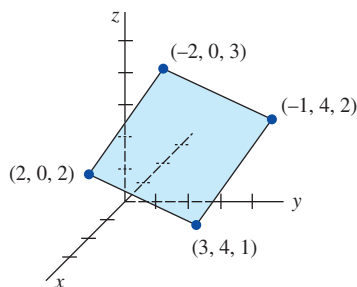
FIGURE 7.4.8 Parallelogram in Problem 46
