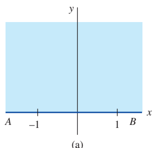
FIGURE 20.4.4 Image of upper half-plane in Example 1
