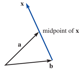
FIGURE 7.1.15 Vector \mathbf{x} in Problem 38
