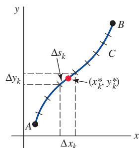
FIGURE 9.8.3 Sample point in k th subarc
