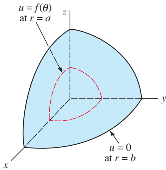
FIGURE 14.3.3 Hollow sphere in Problem 5
