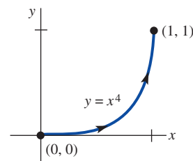
FIGURE 9.9.7 Curve for Problem 17
