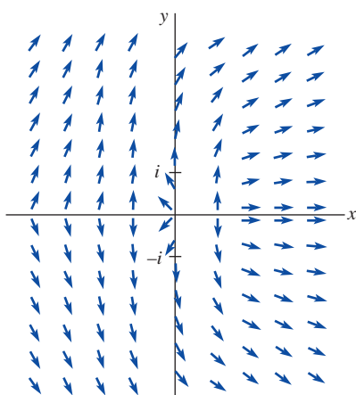
FIGURE 17.6.4 w = \text{Ln } z as a flow
