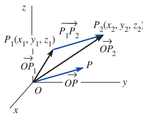
FIGURE 7.2.7 \overrightarrow{OP} and \overrightarrow{P_1P_2} are the same vector
