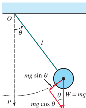
FIGURE 3.11.3 Simple pendulum
