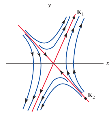
FIGURE 11.2.5 Saddle point
