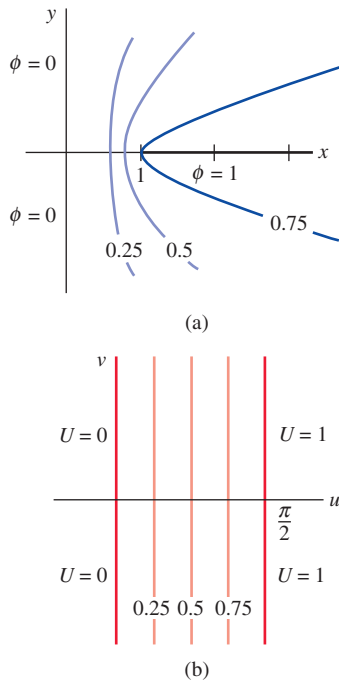
FIGURE 20.6.1 Images of boundary conditions in Example 3
