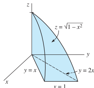
FIGURE 9.R.1 Solid for Problem 33
