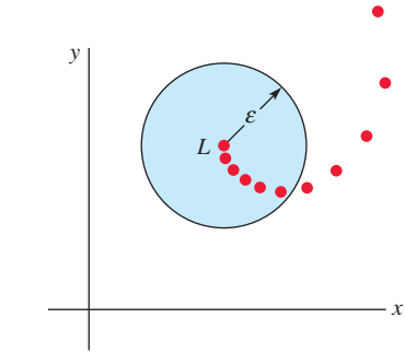
FIGURE 19.1.1 If \{z_n\} converges to L , all but a finite number of terms are in any \varepsilon -neighborhood of L
