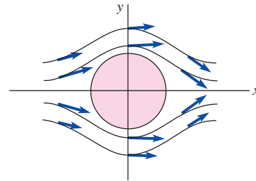
FIGURE 9.7.9 Vector field in Problem 43
