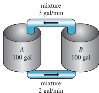
FIGURE 2.9.6 Mixing tanks in Problem 9
