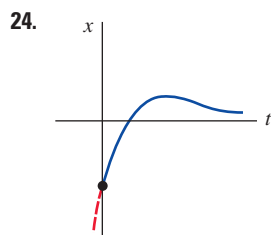
FIGURE 3.8.21 Graph for Problem 24
