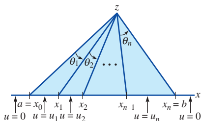
FIGURE 20.5.2 General boundary conditions on y = 0
