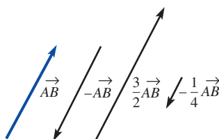
FIGURE 7.1.3 Parallel vectors
