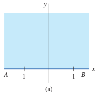
FIGURE 20.4.3 Image of upper half-plane
