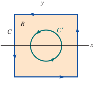
FIGURE 9.12.11 Curves C and C' in Example 6
