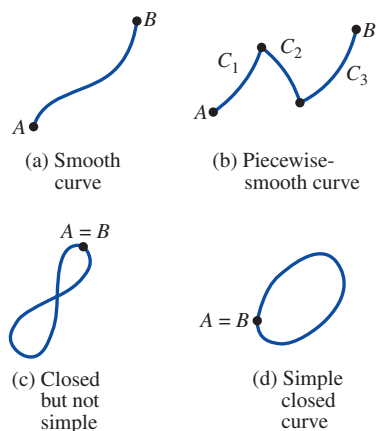
FIGURE 9.8.1 Various curves
