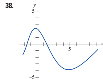
FIGURE 1.2.10 Graph for Problem 38
