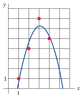
FIGURE 8.16.4 Least squares parabola in Example 3
