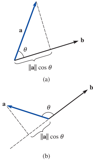
FIGURE 7.3.4 Component of \mathbf{a} on \mathbf{b}
