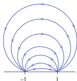
FIGURE 20.6.13 Streamlines in Problem 23
