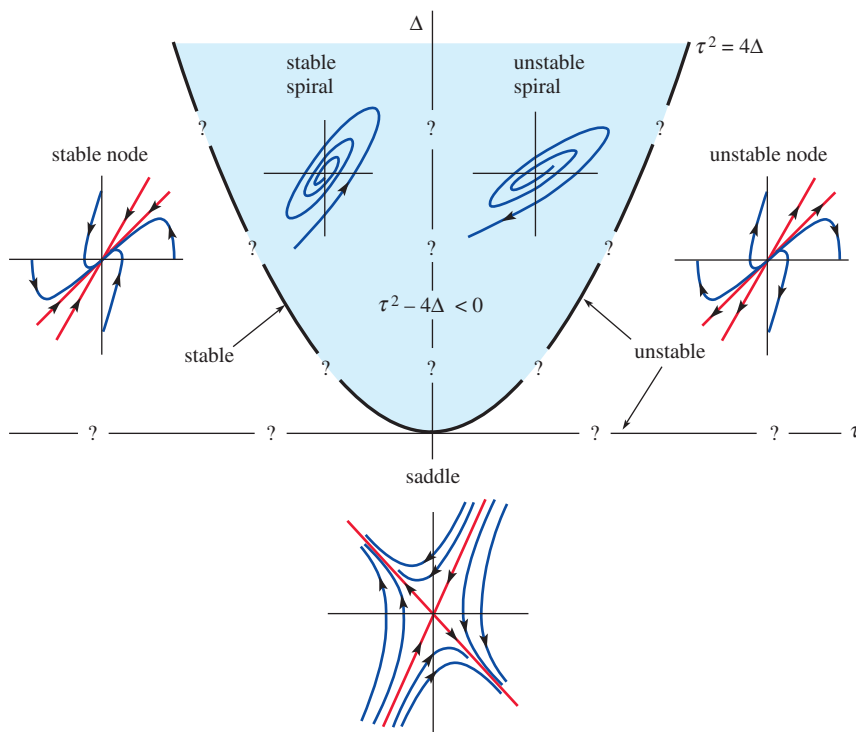
FIGURE 11.3.7 Geometric summary
