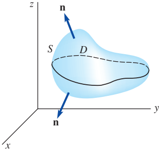
FIGURE 9.16.2 Region D with no vertical side
