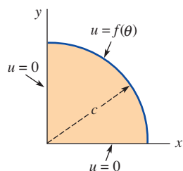
FIGURE 14.1.4 Quarter-circular plate in Problem 7
