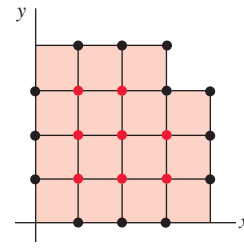
FIGURE 16.1.8 Region in Problem 8
