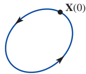
FIGURE 11.1.3 Periodic solution or a cycle
