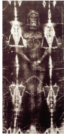
FIGURE 2.7.9 Shroud image in Problem 12
