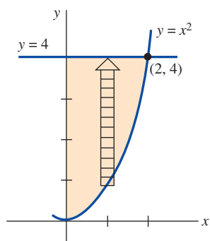
FIGURE 9.10.7 Summation in y -direction in (a); summation in x -direction in (b)
