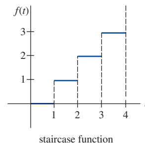
FIGURE 4.3.19 Graph for Problem 62
